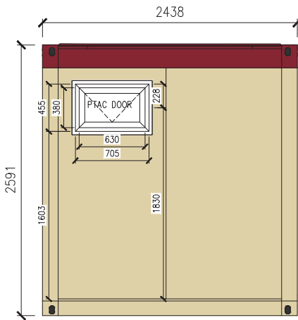
VIEW B
