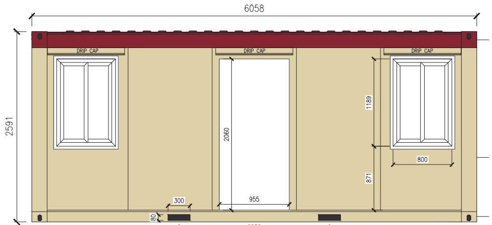
VIEW A
